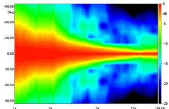
Vertical Beamwidth
