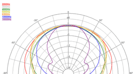
Horizontal Polar Pattern
